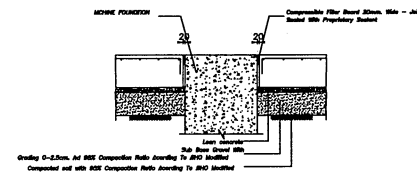
DETAIL
