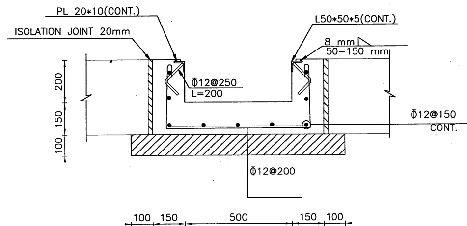
SECTION E-E
